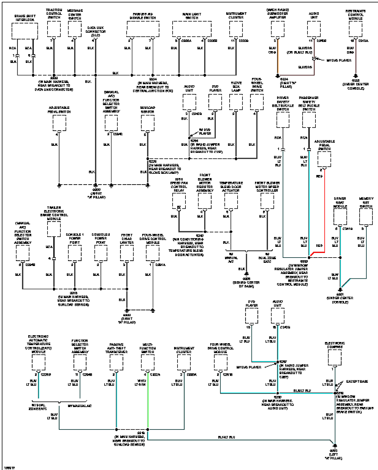
Fig. 29: Ground Distribution Circuit (2 of 4)
