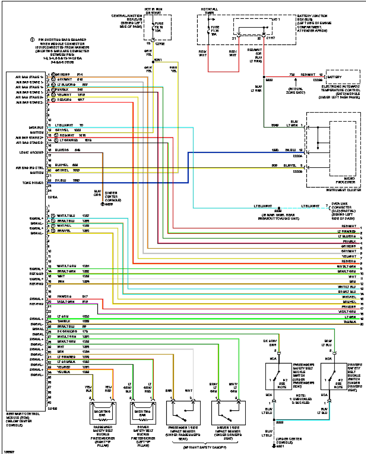
Fig. 63: Supplemental Restraints Circuit (1 of 2)
