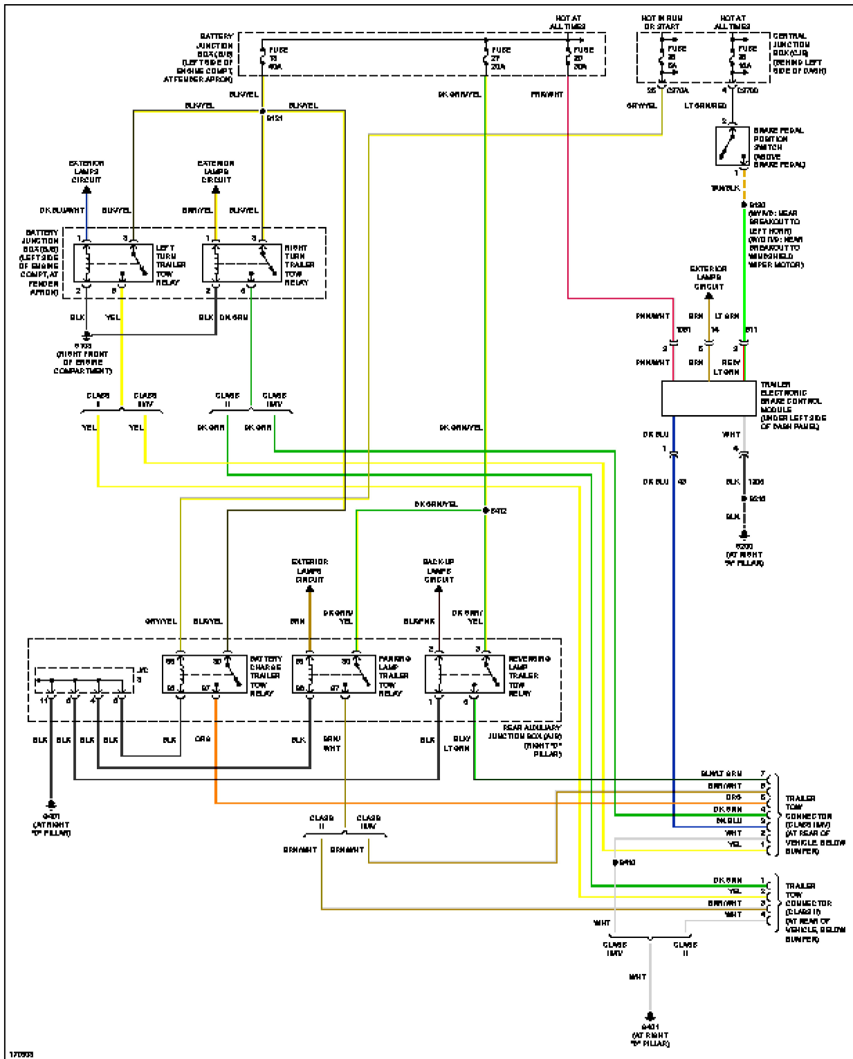
Fig. 26: Trailer Tow Circuit, Early Production
