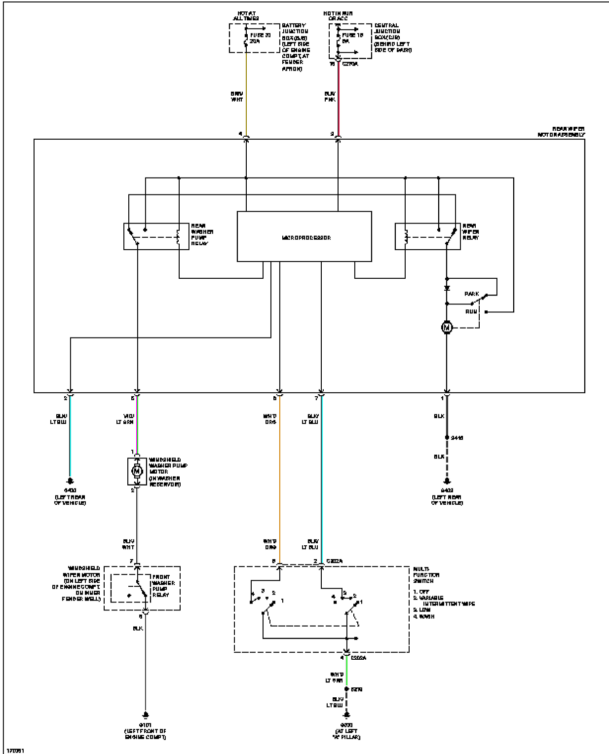
Fig. 71: Rear Washer/Wiper Circuit
