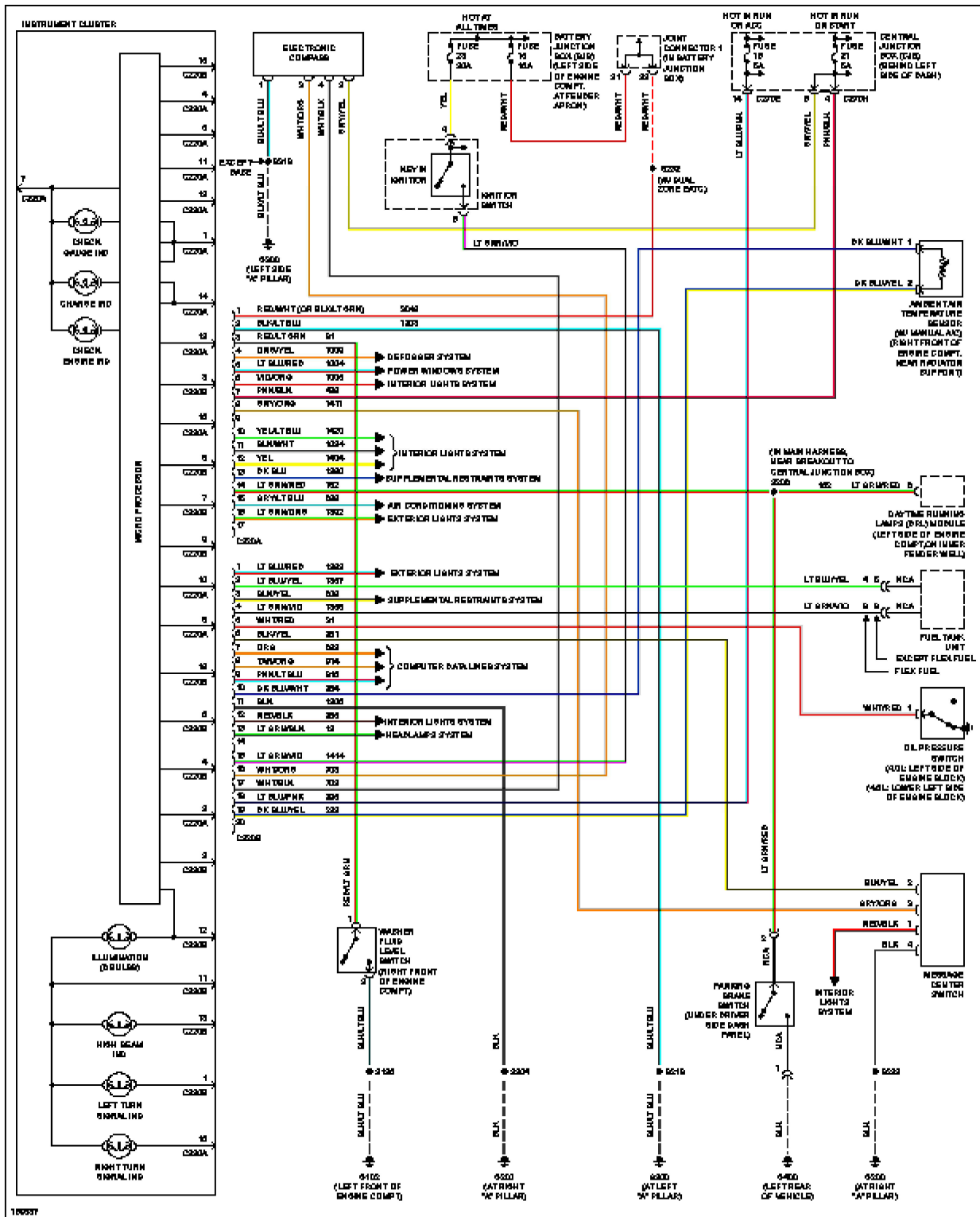
Fig. 35: Instrument Cluster Circuit
