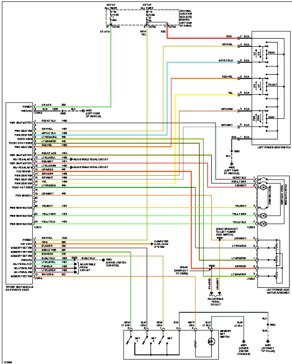
Fig. 41: Driver's Memory Seat Circuit
