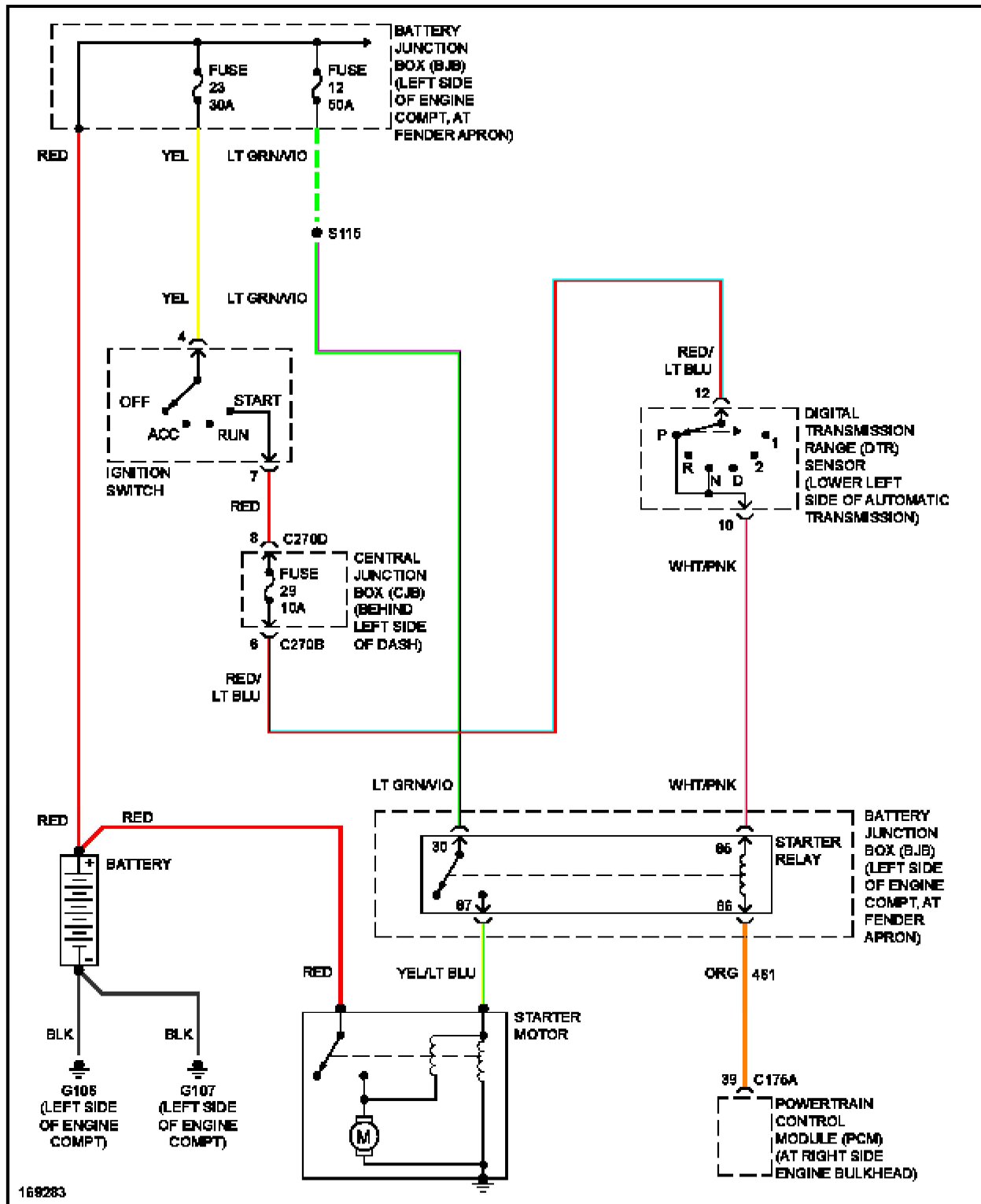
Fig. 62: Starting Circuit
