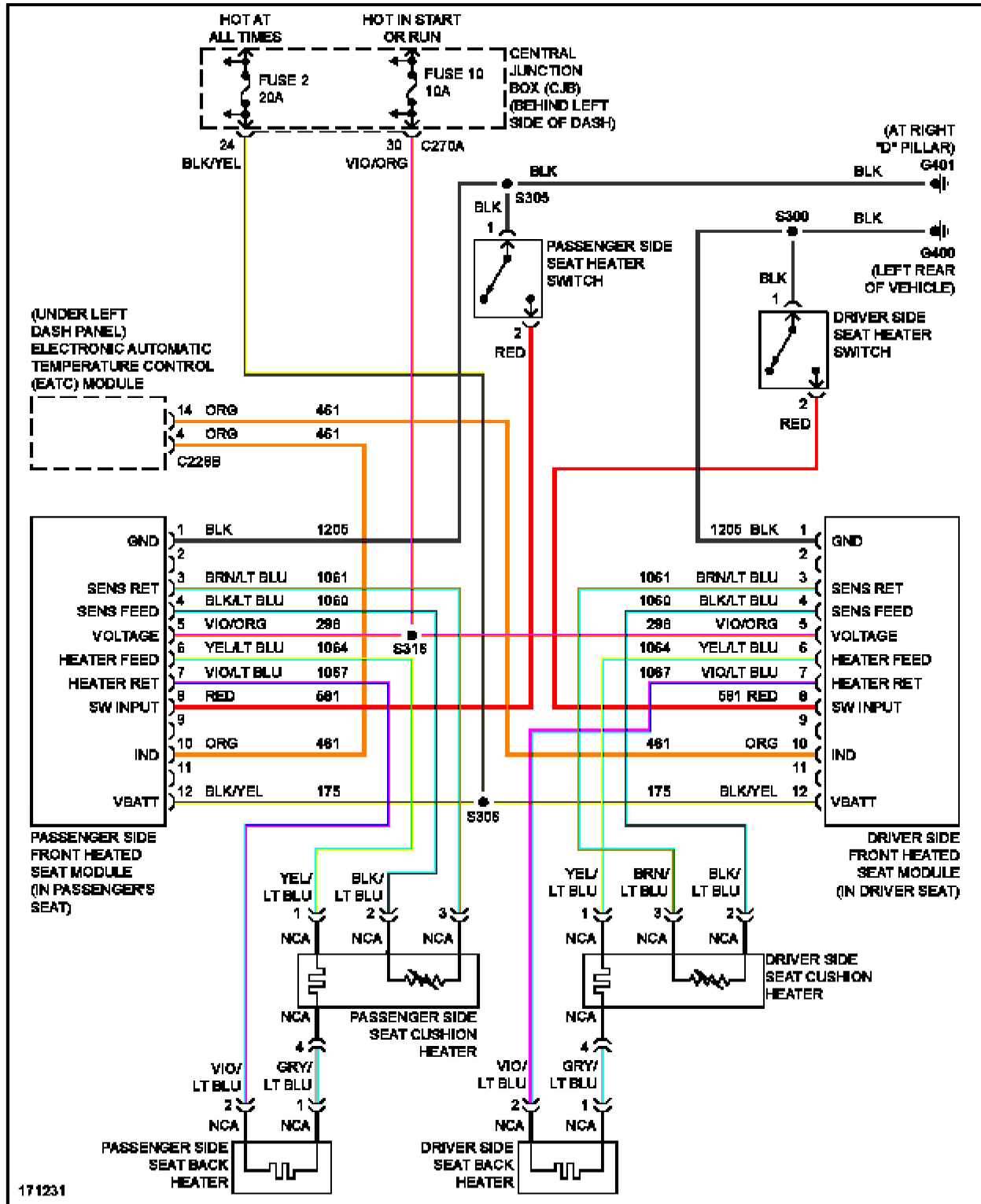
Fig. 52: Heated Seats Circuit, Early Production
