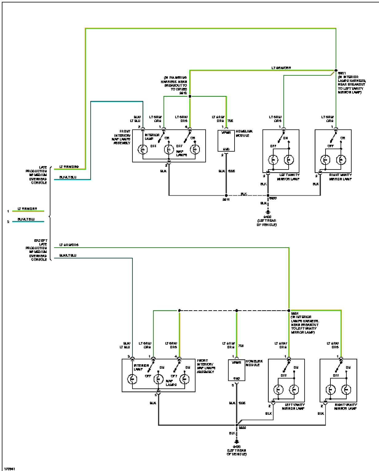
Fig. 38: Courtesy Lamps Circuit, Except Base (2 of 2)
