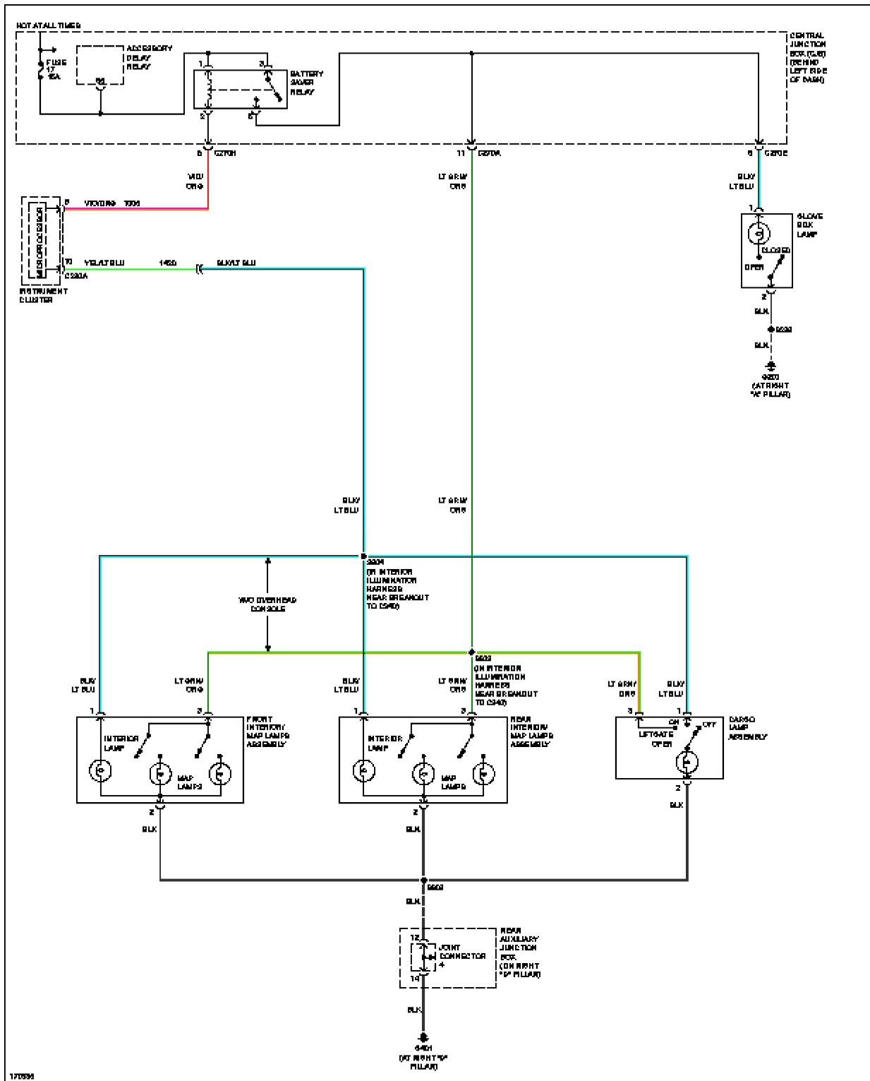
Fig. 36: Courtesy Lamps Circuit, Base
