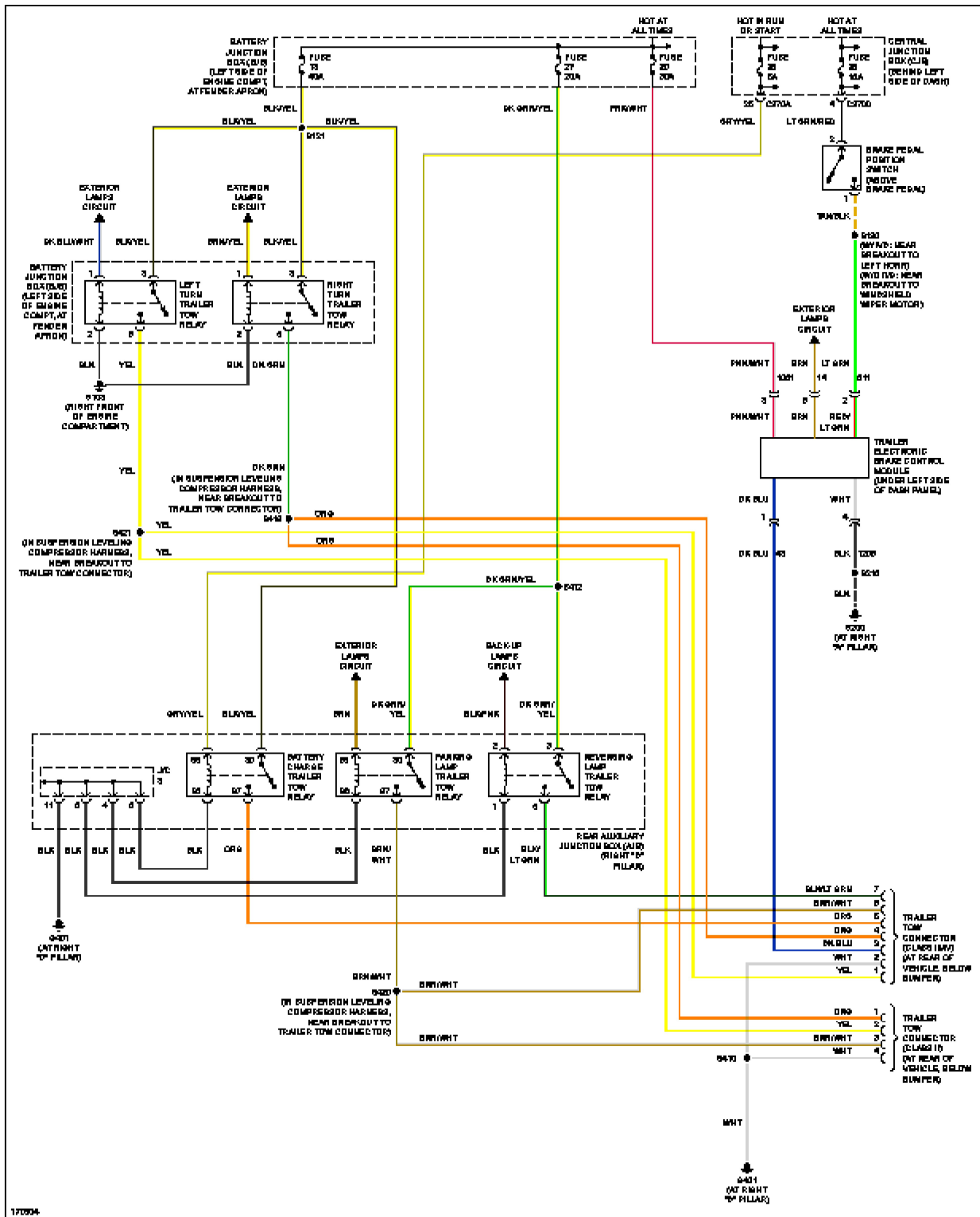
Fig. 27: Trailer Tow Circuit, Late Production
