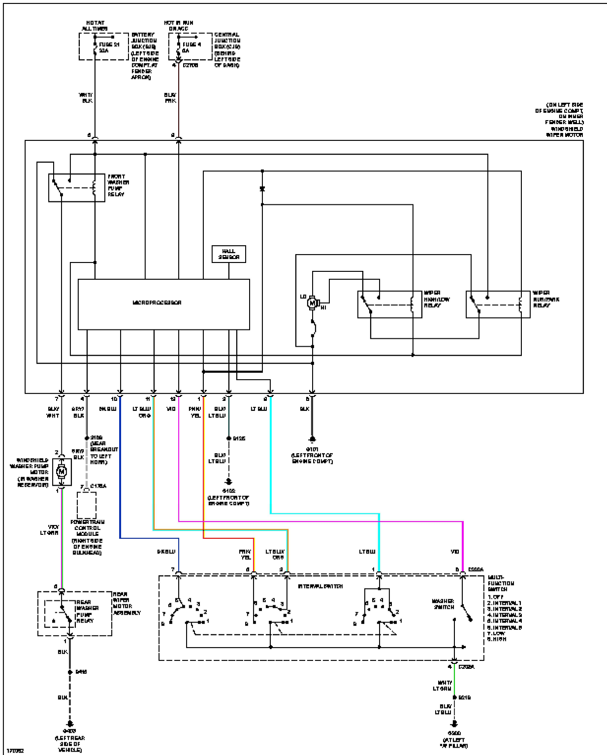
Fig. 70: Front Wiper/Washer Circuit
