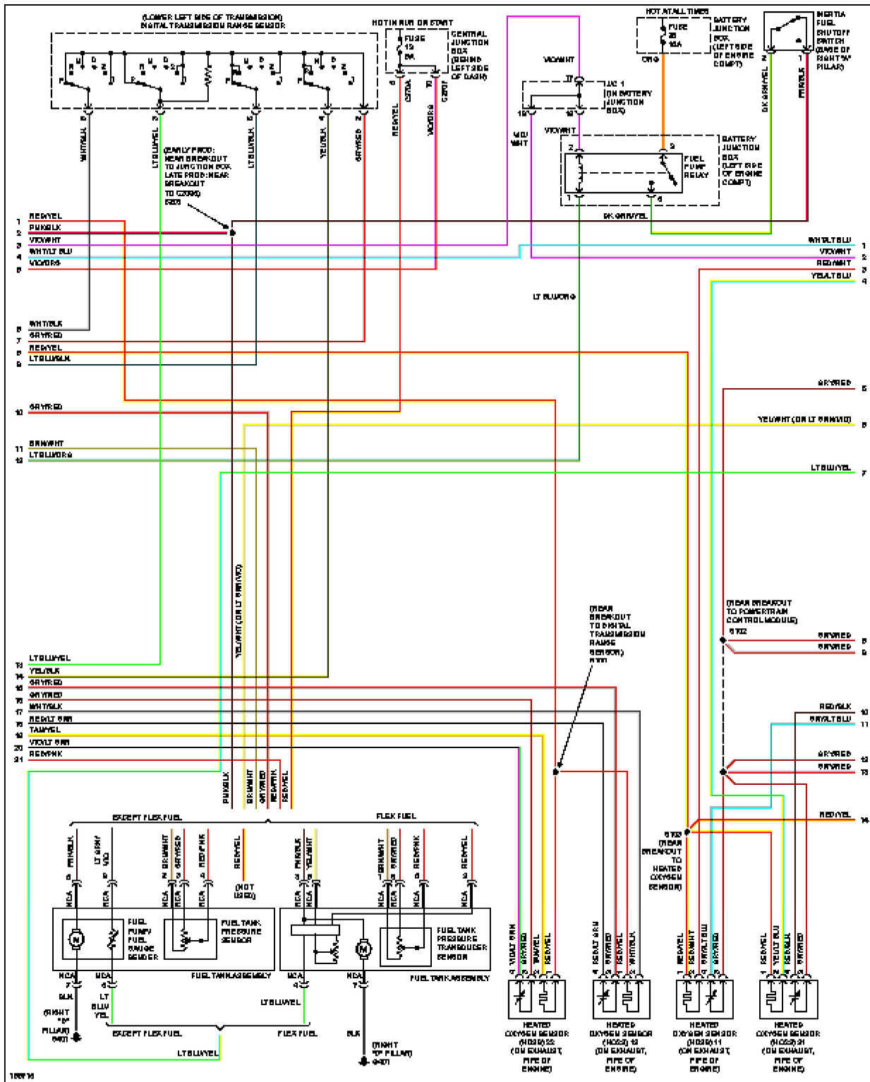
Fig. 17: 4.0L, Engine Performance Circuit (3 of 4)
