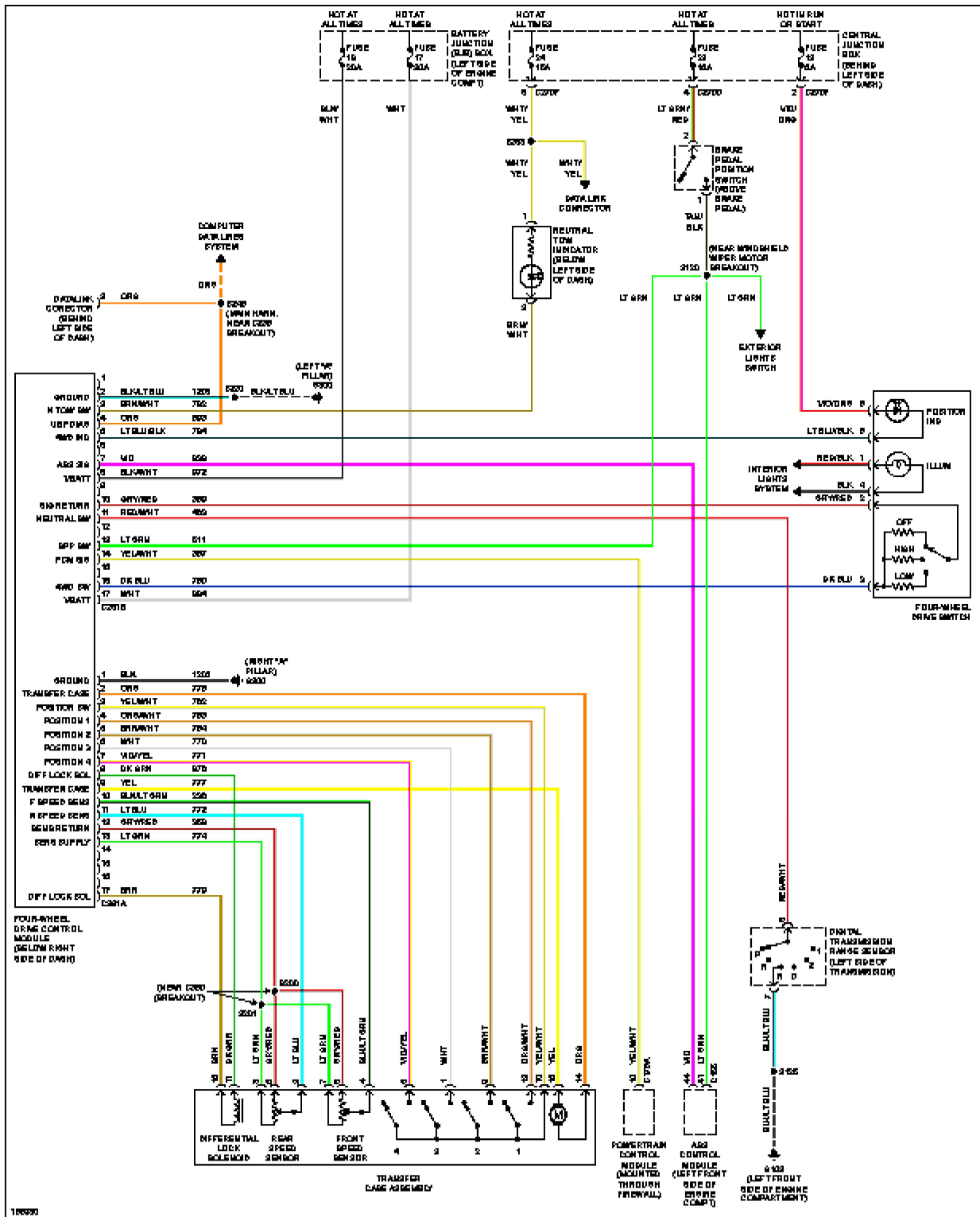
Fig. 66: 4WD Circuit, W/O Traction Control
