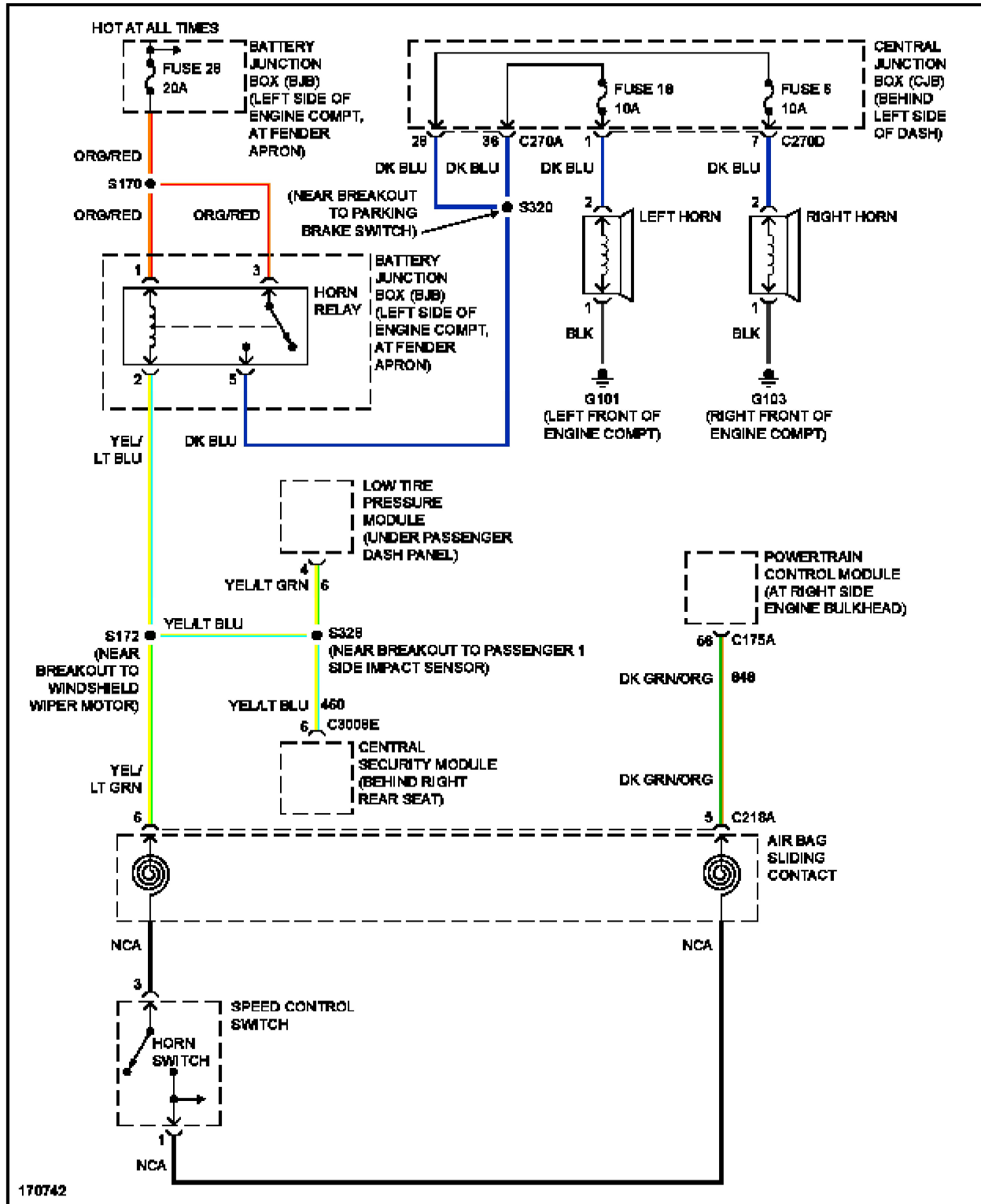
Fig. 34: Horn Circuit
