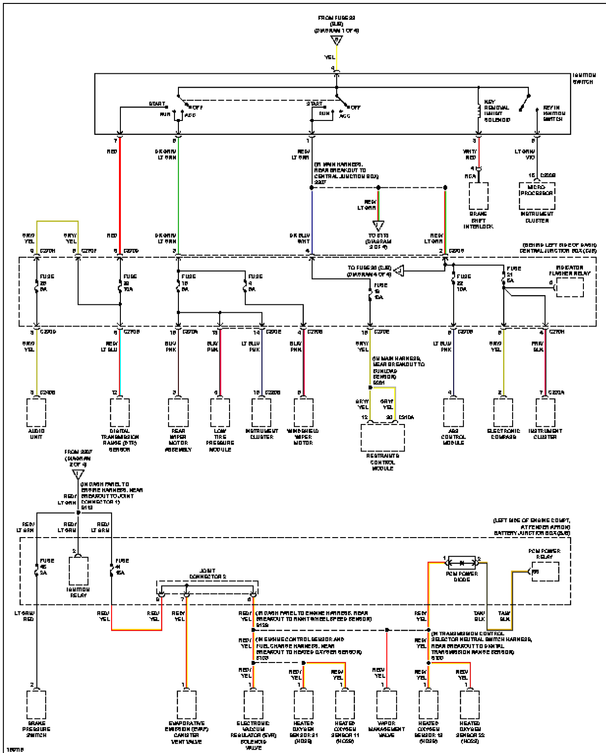
Fig. 44: Power Distribution Circuit (2 of 4)
