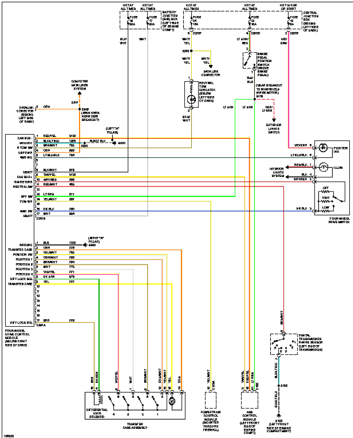
Fig. 65: 4WD Circuit, W/ Traction Control
