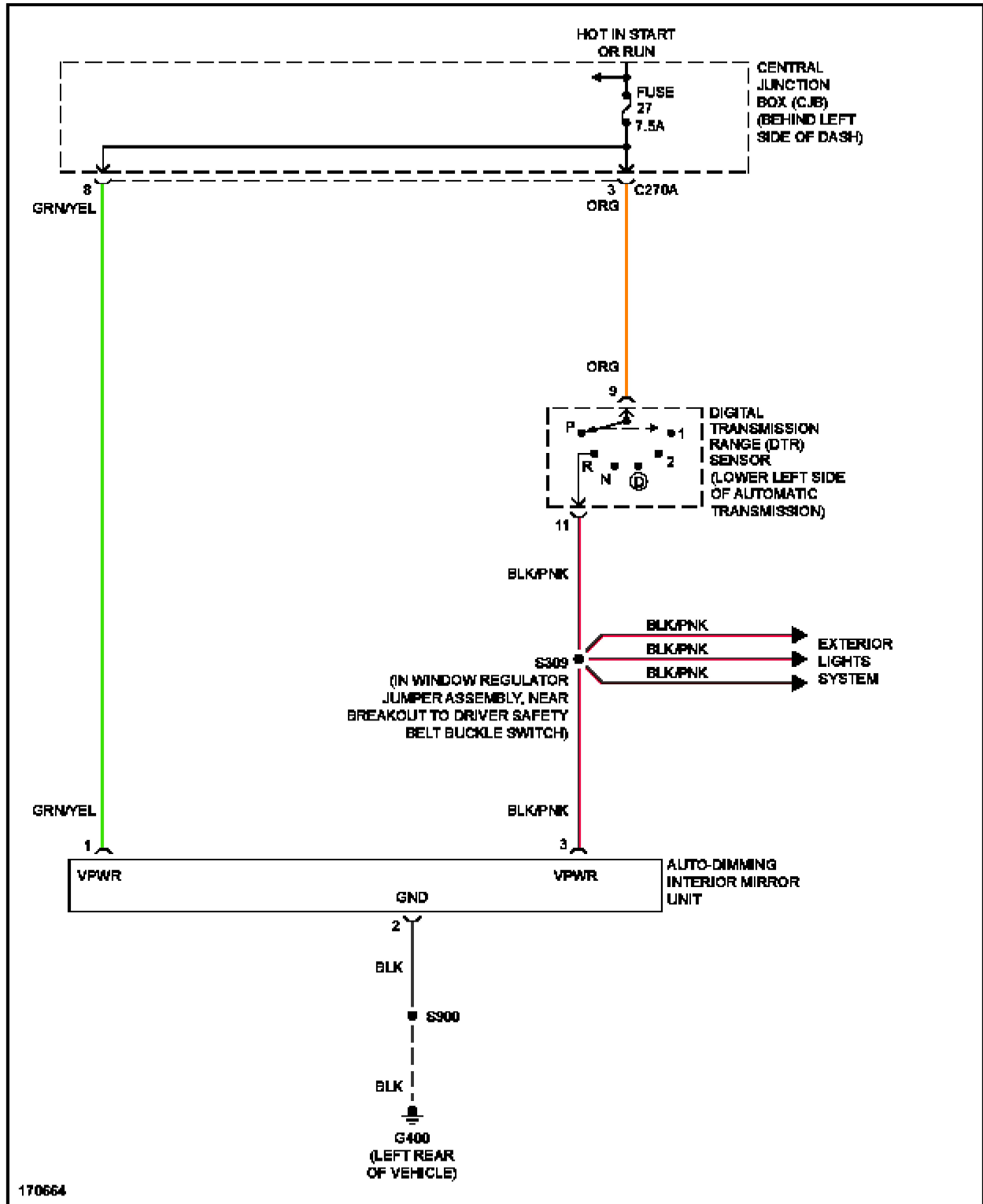
Fig. 48: Electronic Day/Night Mirror Circuit
