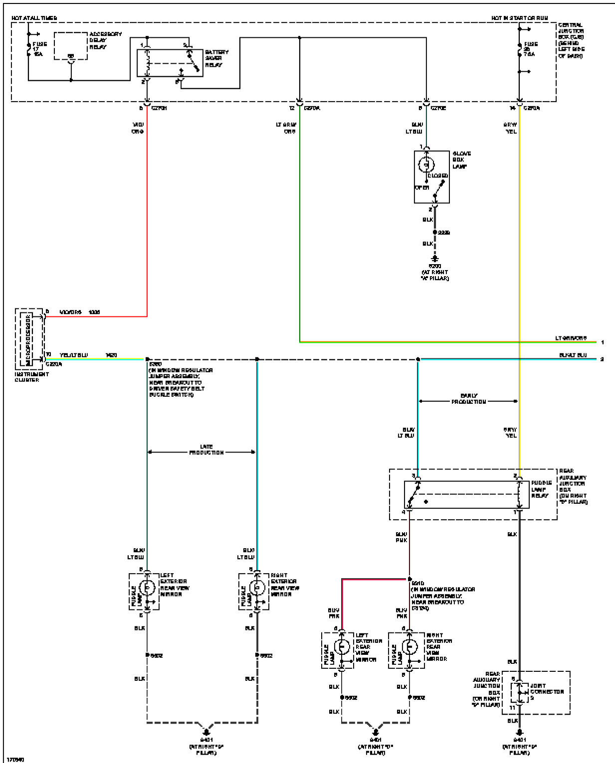
Fig. 37: Courtesy Lamps Circuit, Except Base (1 of 2)
