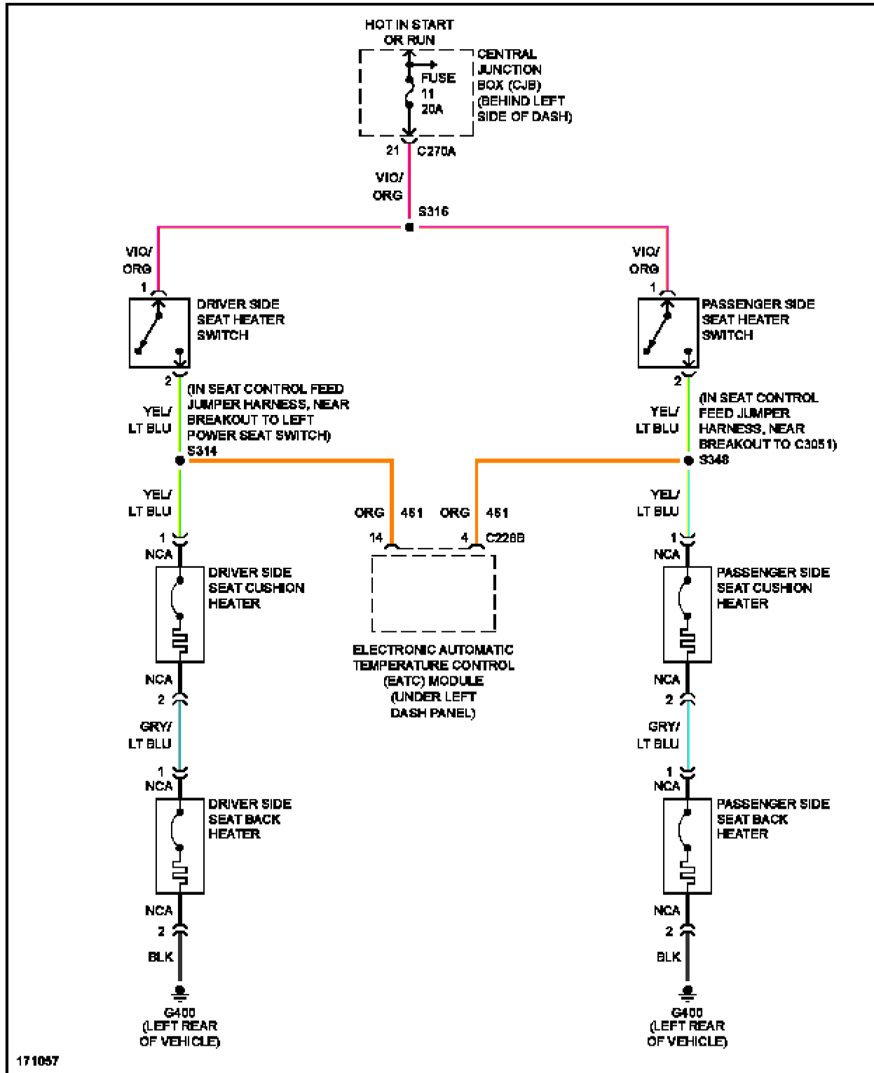
Fig. 53: Heated Seats Circuit, Late Production
