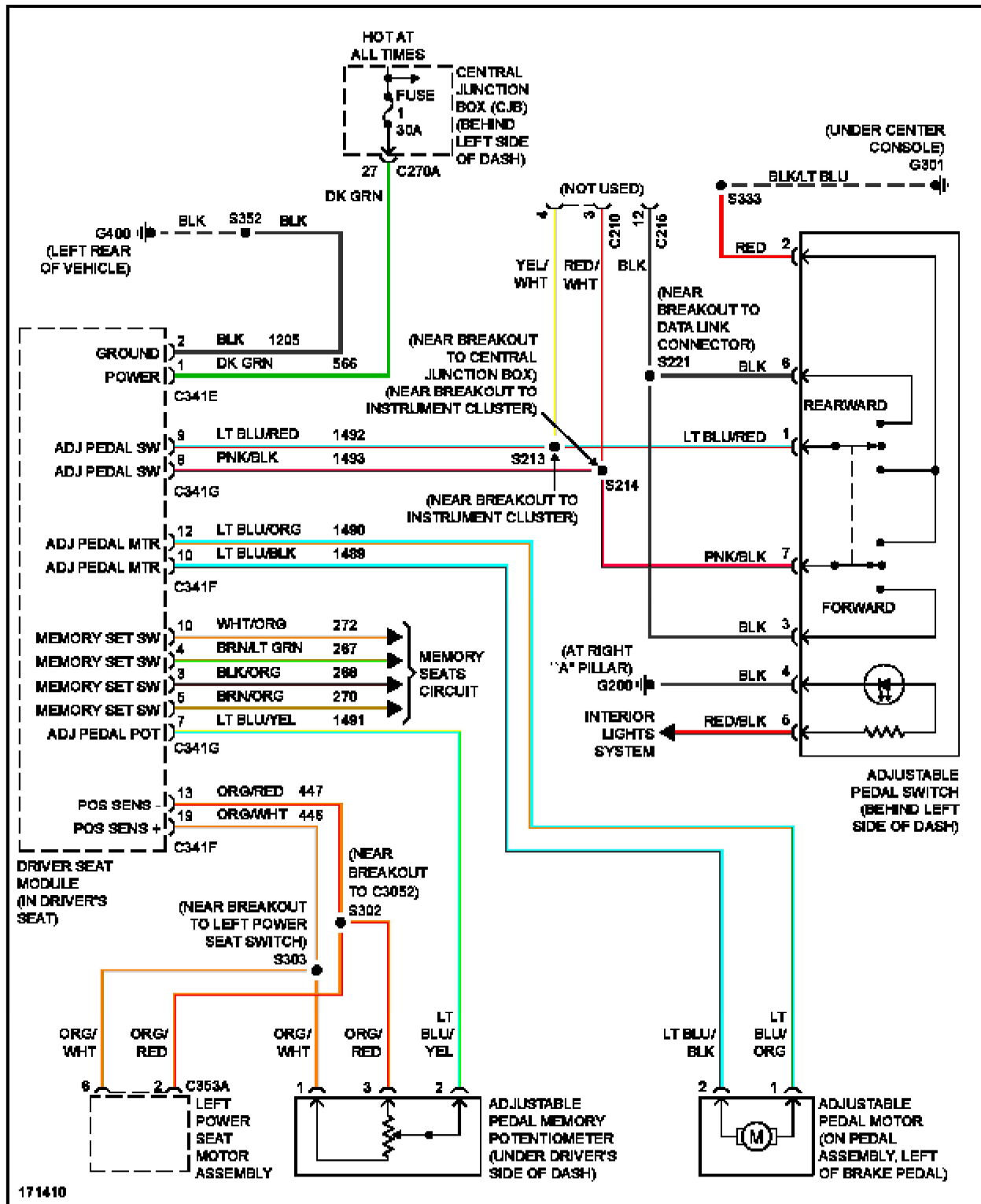
Fig. 40: Adjustable Pedal Circuit
