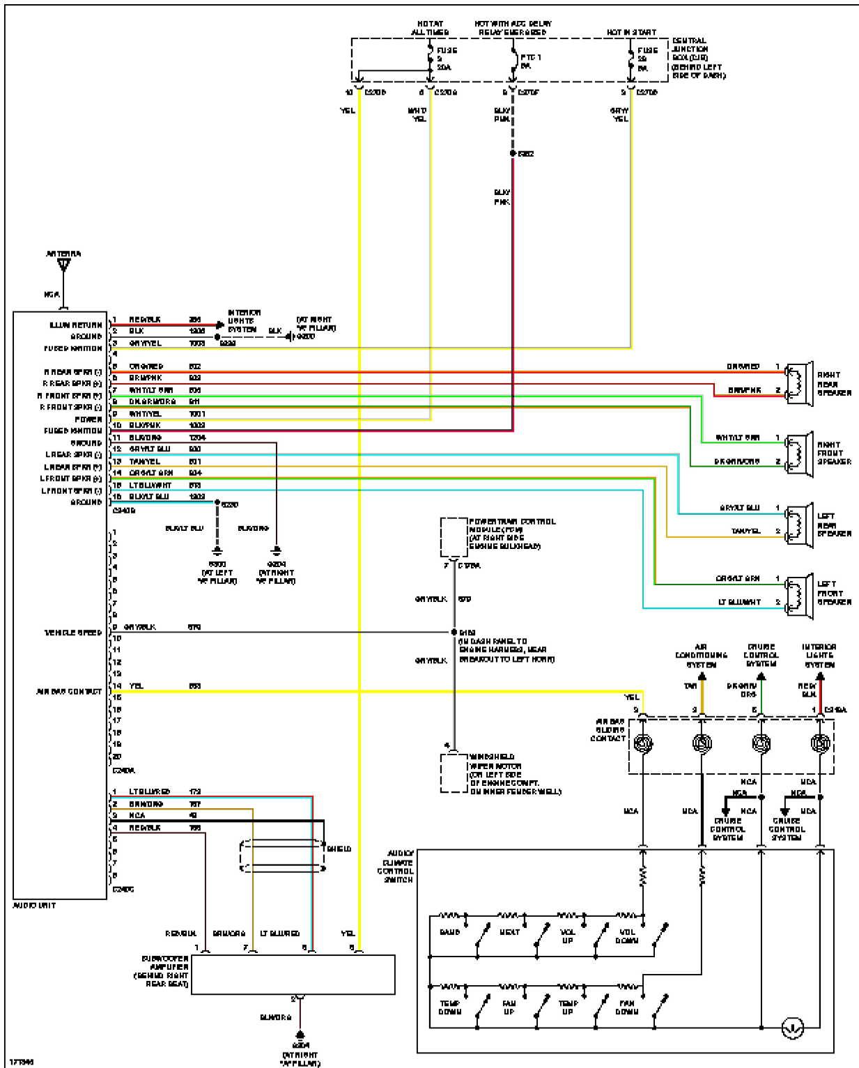
Fig. 58: Premium Sound Radio Circuit
