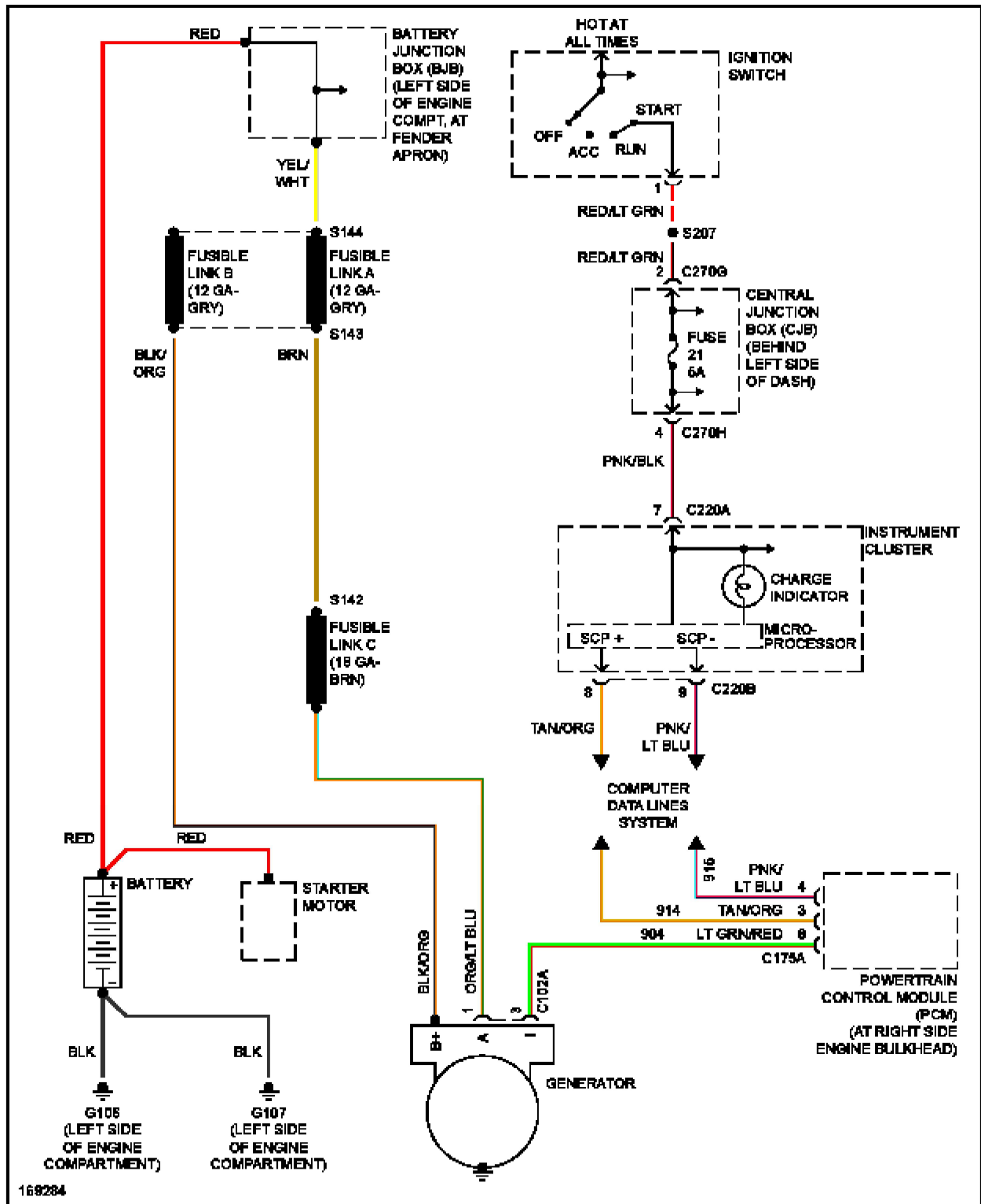
Fig. 61: Charging Circuit
