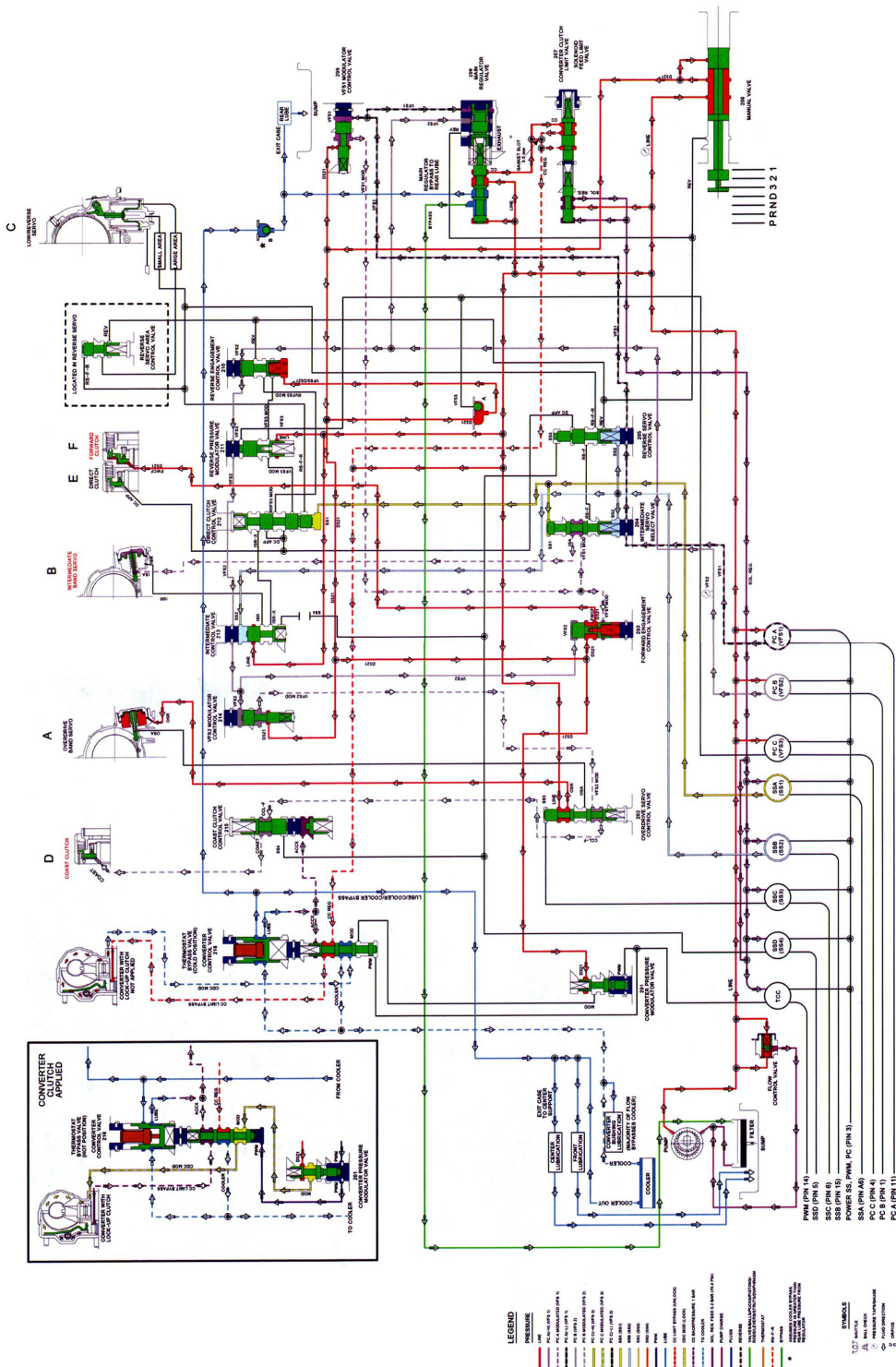
Fig. 9: Manual 3rd Gear Courtesy of FORD MOTOR CO.
