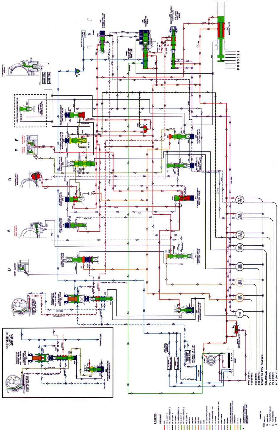
Fig. 7: 5th Gear Courtesy of FORD MOTOR CO.
